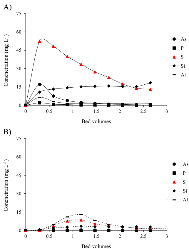
Fig. 6 Elution curves of competing elements from the column with 2.0 M NaOH in a test 1 with operating BDRA neat residue leachate (pH 13) and b test 2 with post-closure effluent (pH 11.5)
